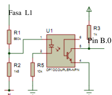
Gambar 5. Optocoupler NPN-4N35
